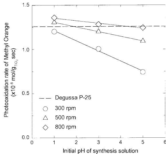
Fig. 6. Comparison of photooxidation rate of methyl orange using the TiO 2 powders prepared by hydrothermal method: volume 0.1 L, concentration 30 ppm, air flow rate 0.5 L/min.
